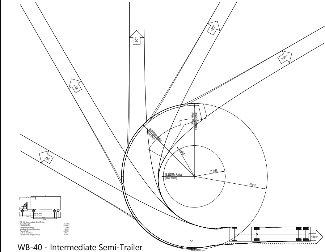
WB-40 - Intermediate Semi-Trailer Notes: Turns based upon front axle following a circular arc starting tangentially. Vehicle Tracking V24.00.2660/20230214 (C) Autodesk, Inc. www.autodesk.com
