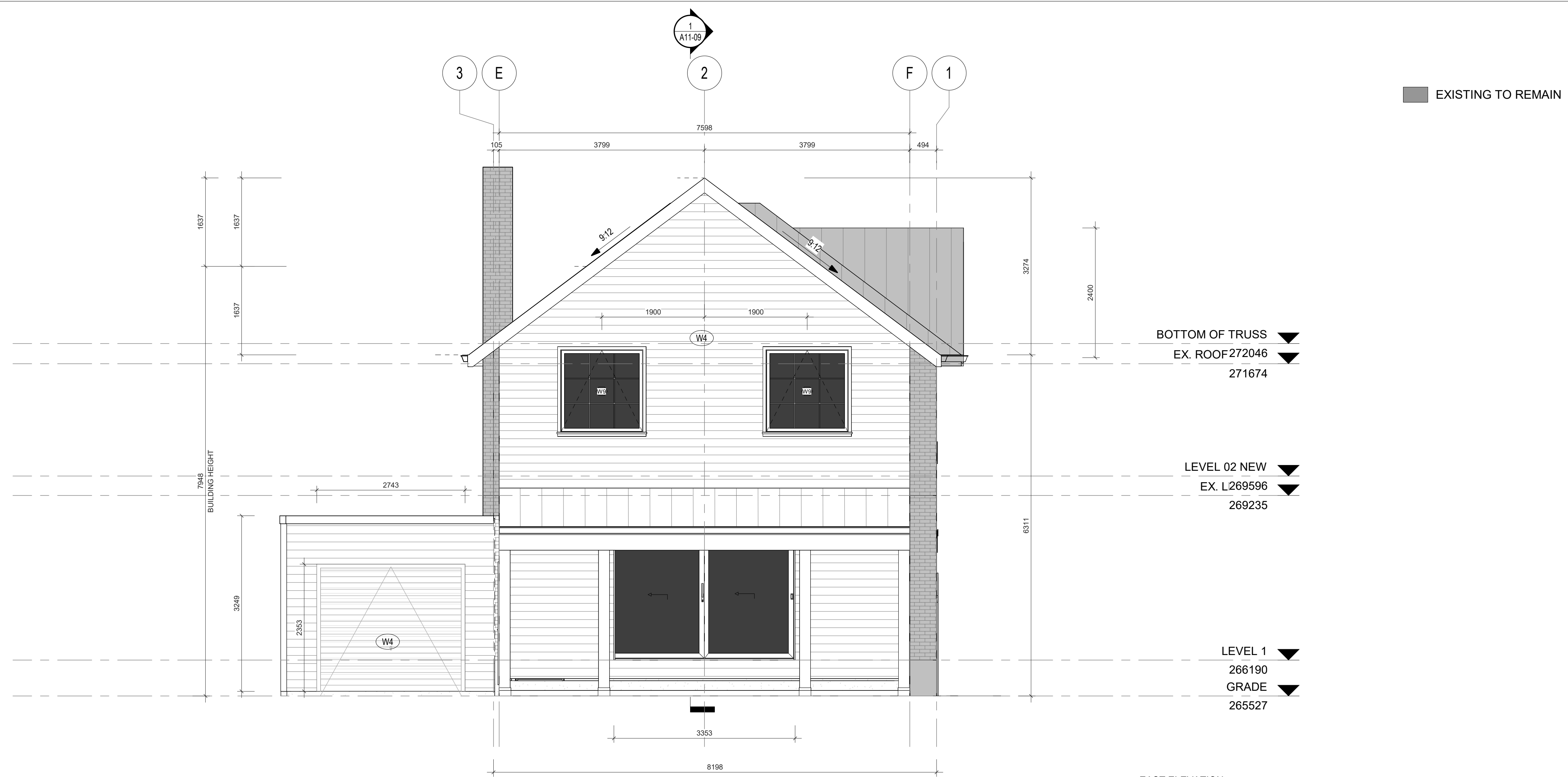
1 EAST ELEVATION 1:50
