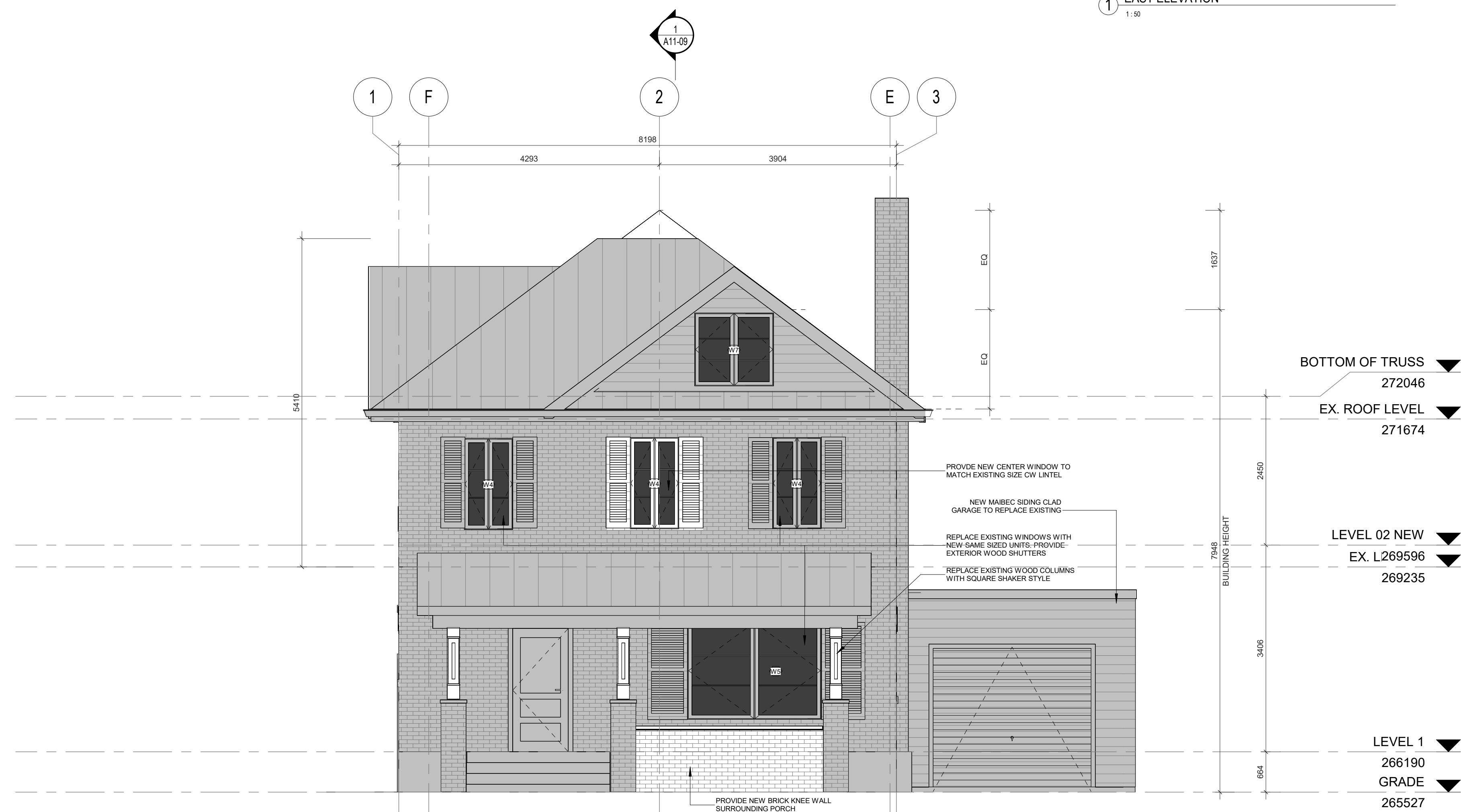
2 WEST Elevation 1:50
