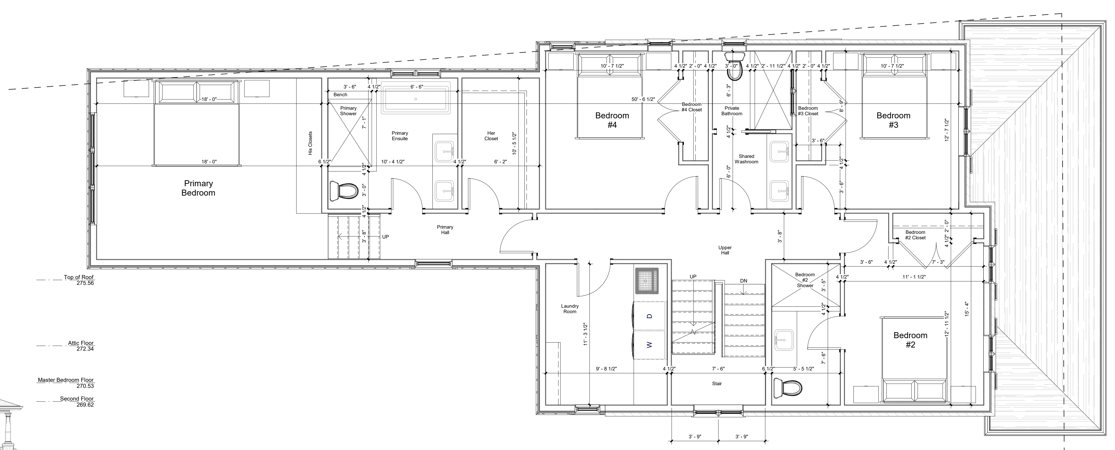
1 Second Floor - Plan 1/4" = 1'-0"
