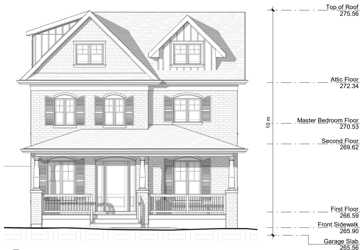
3 East Elevation 1/8" = 1'-0"
