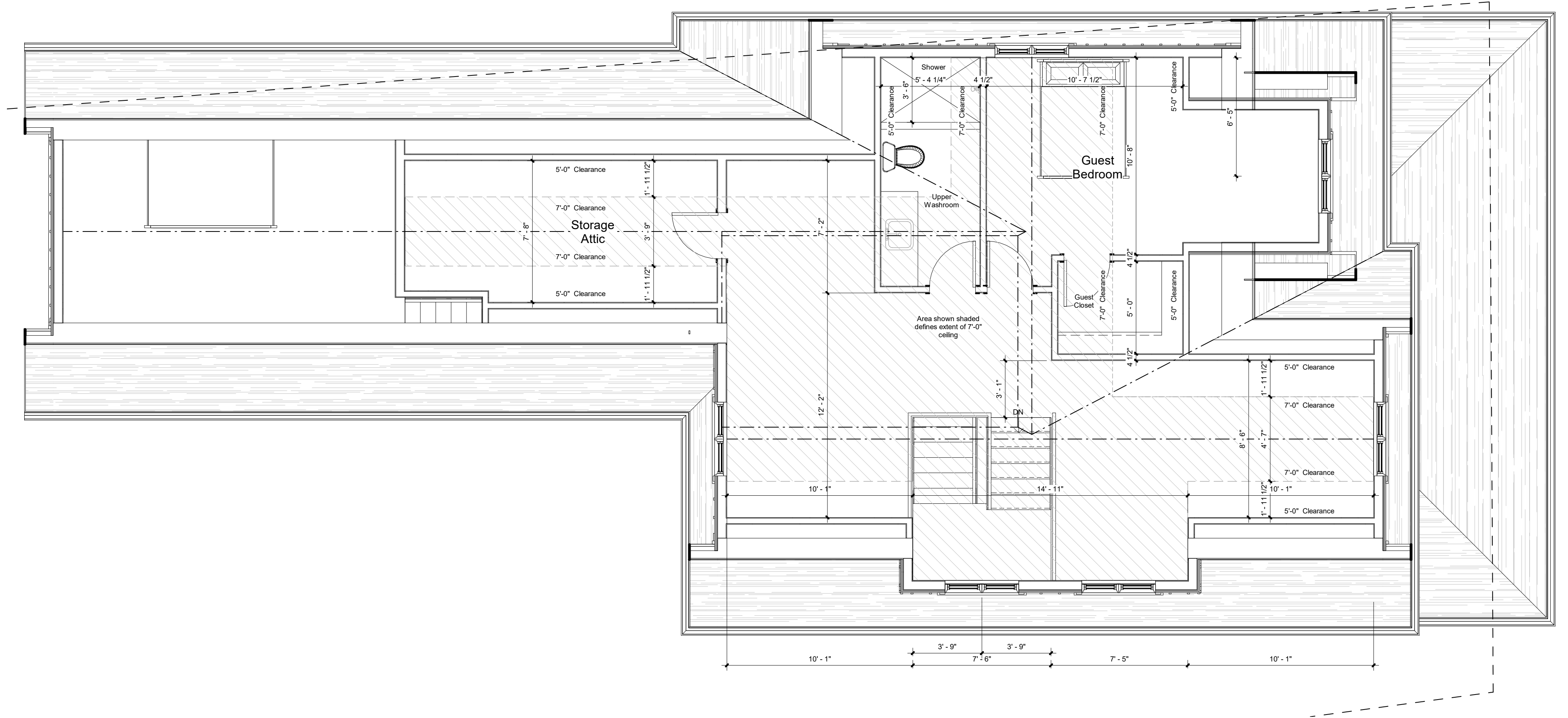
2 Attic Floor 1/4" = 1'-0"
